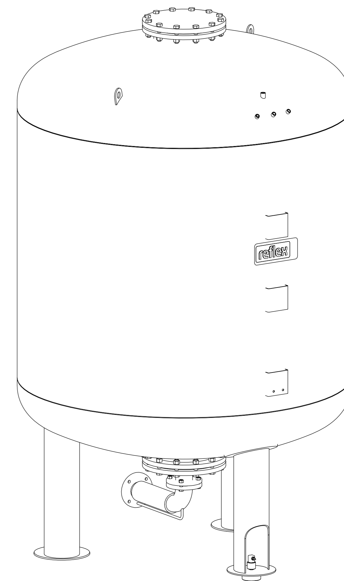
Isometric view
