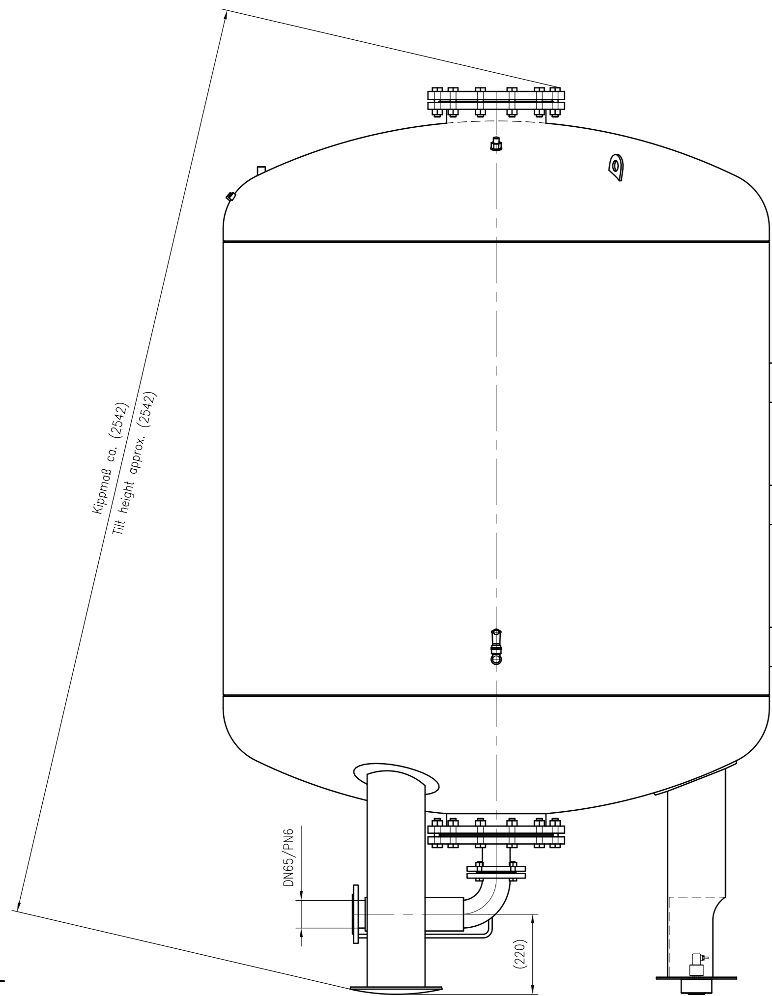
Side view
