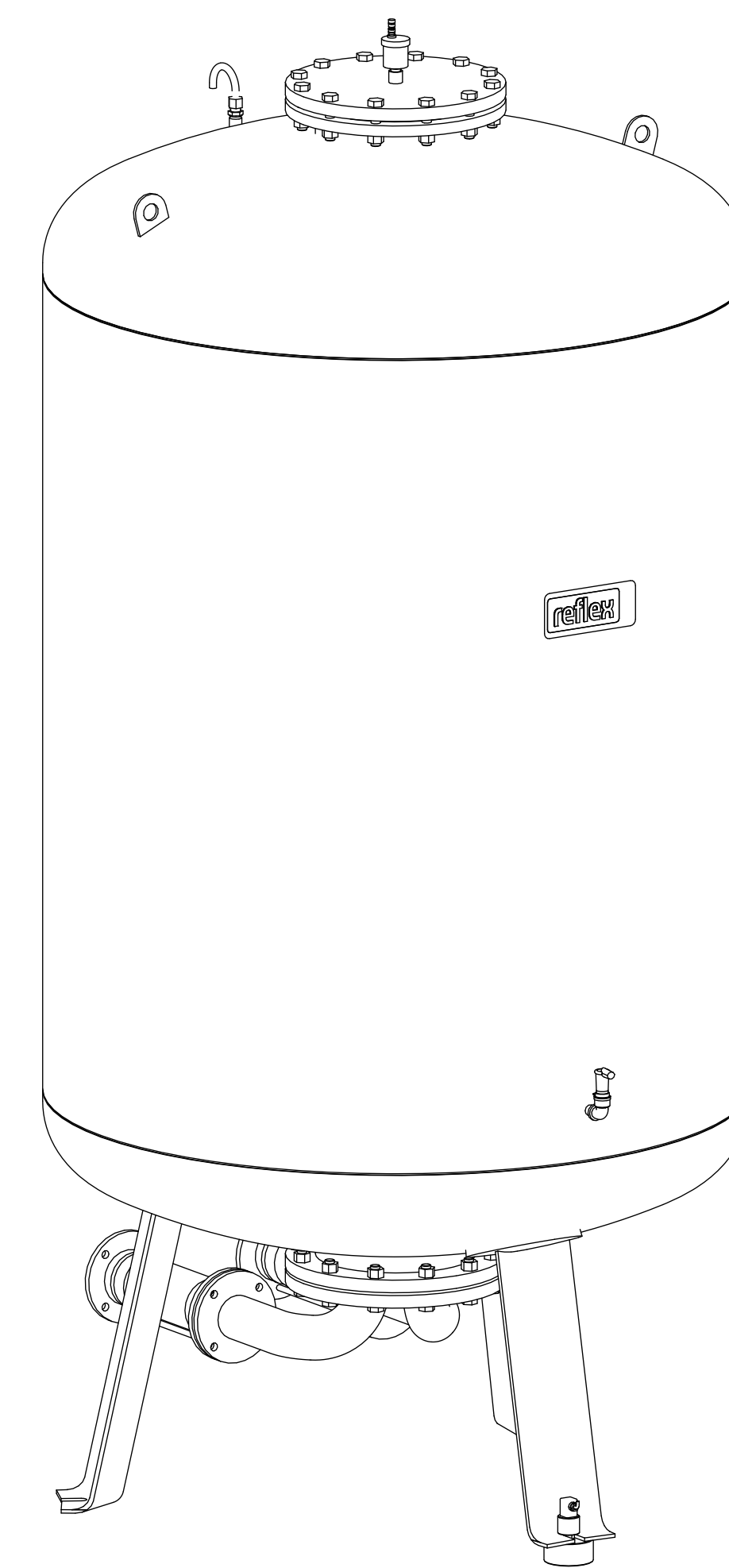
Isometric view
