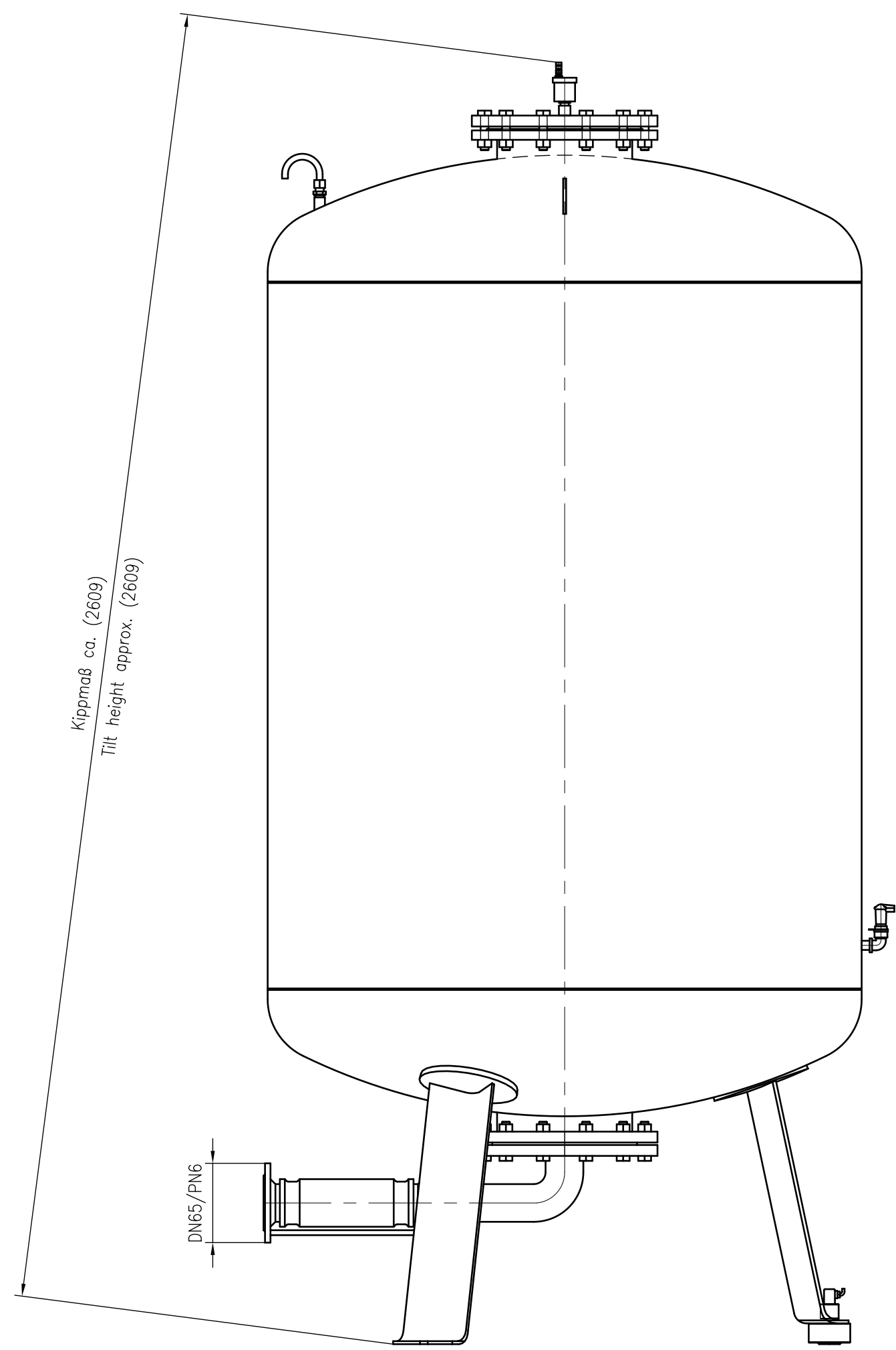
Side view
