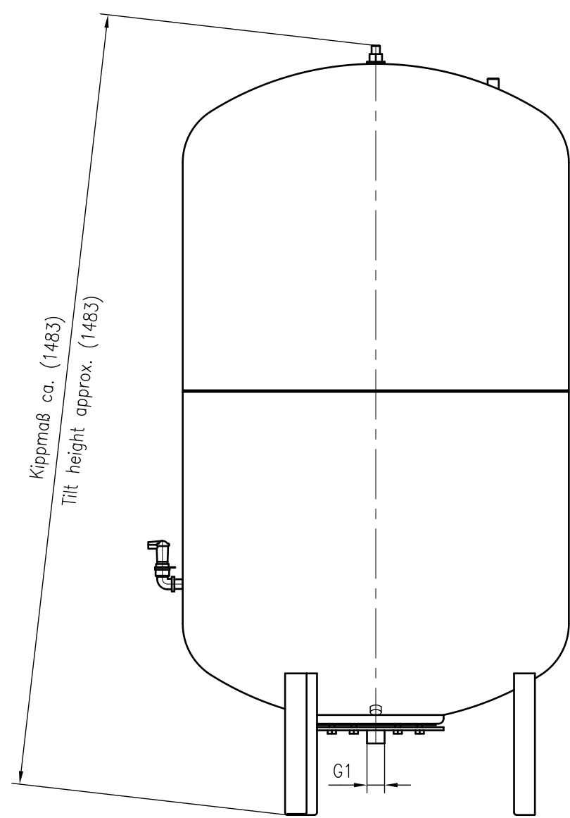
Side view
