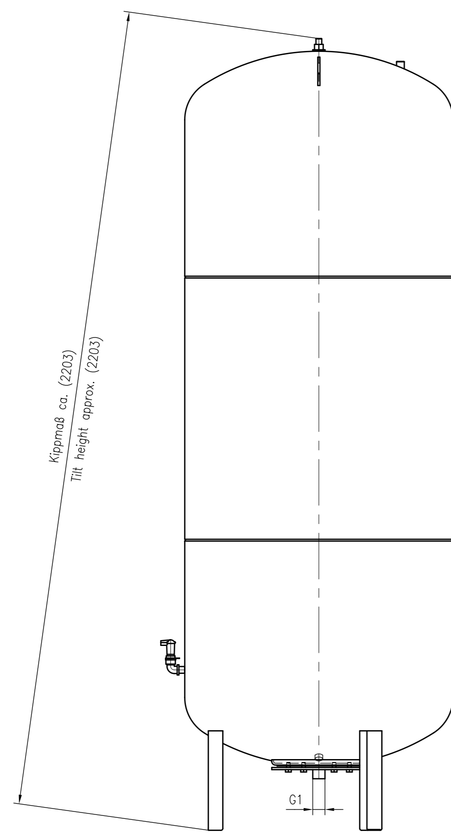
Side view
