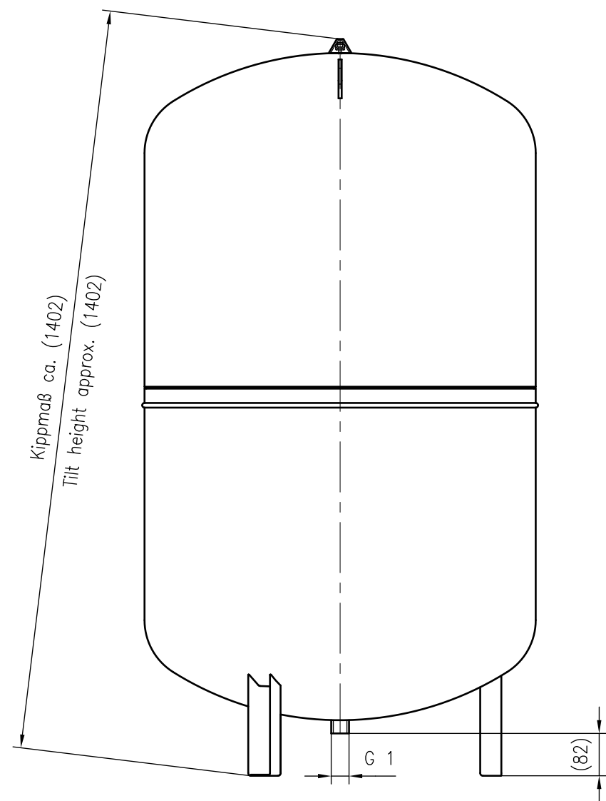
Side view
