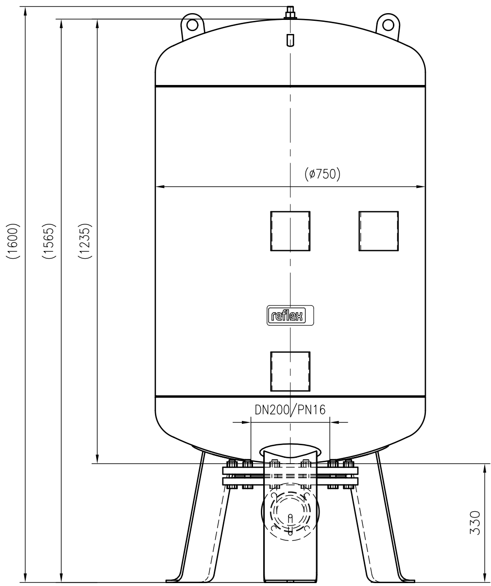
Front view
