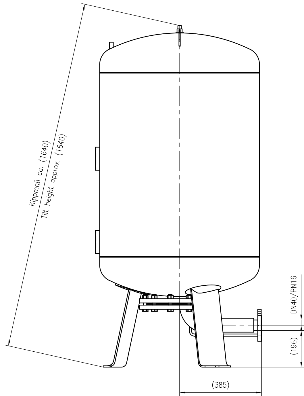
Side view
