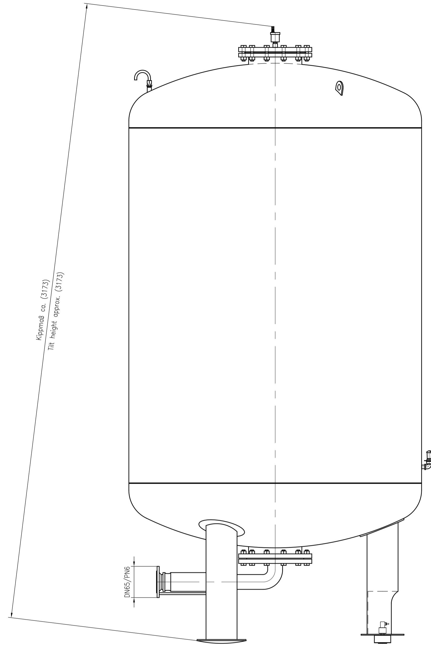
Side view
