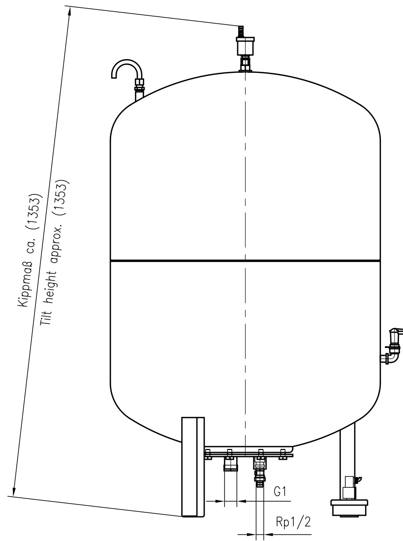
Side view
