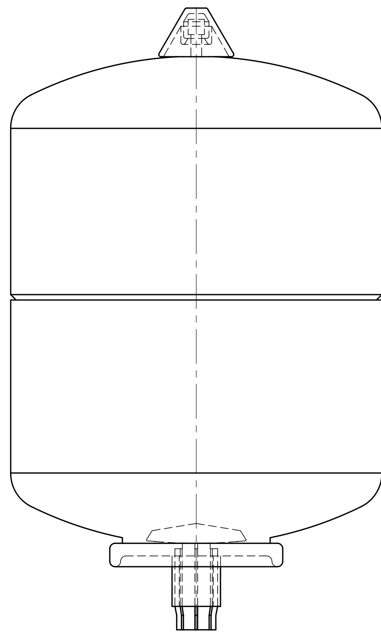
Side view
