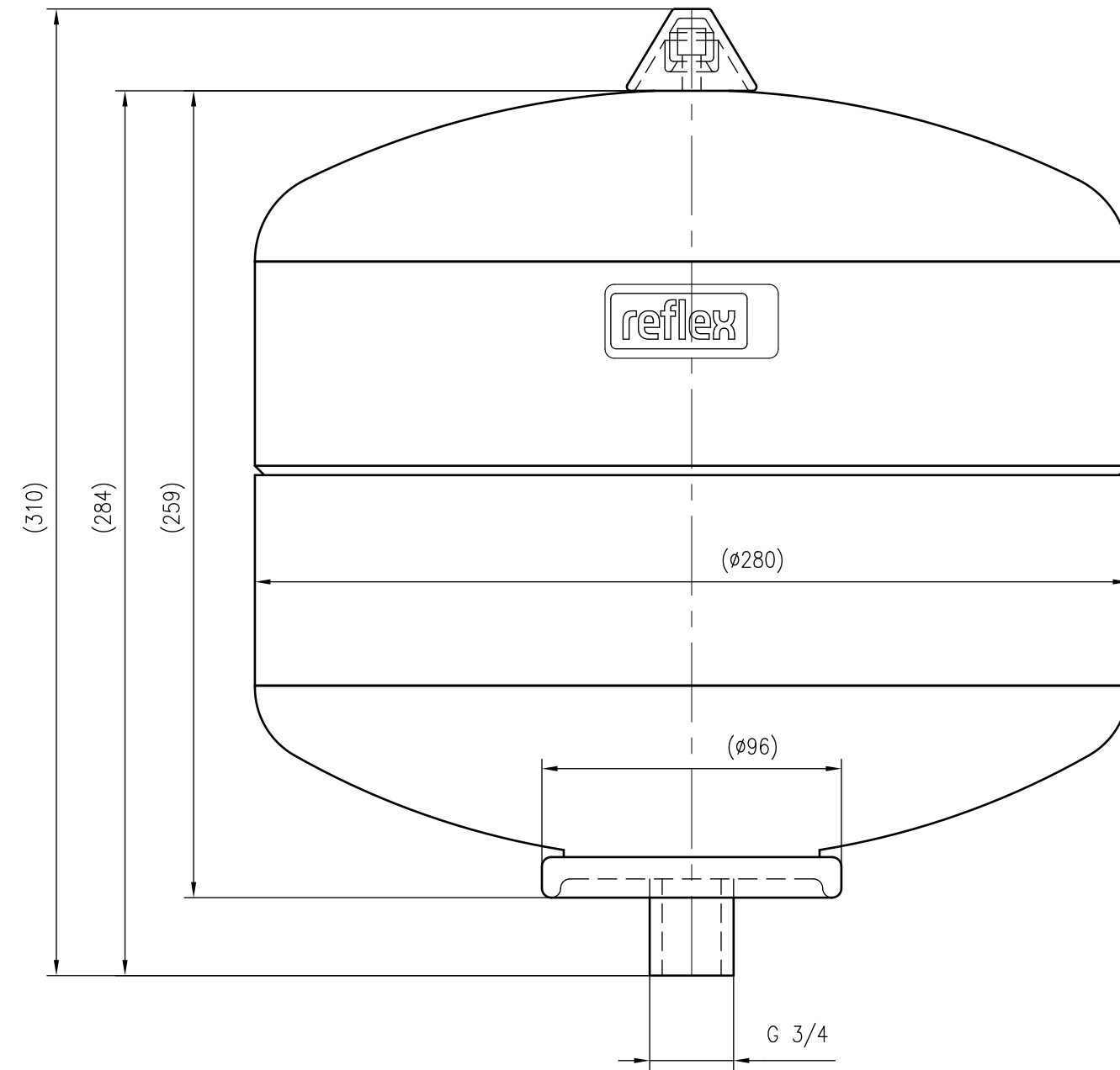
Front view
