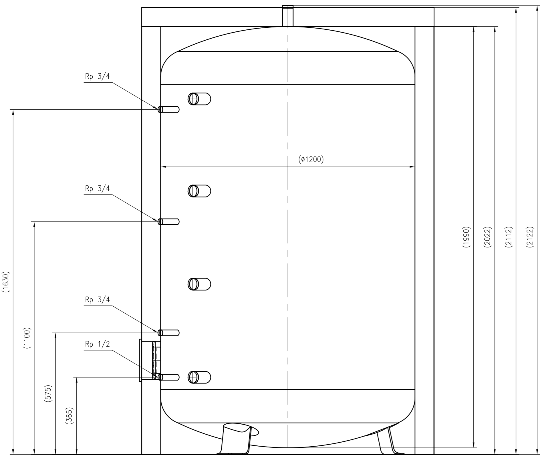
Side view
